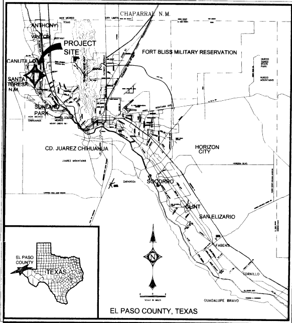
VICINITY MAP
