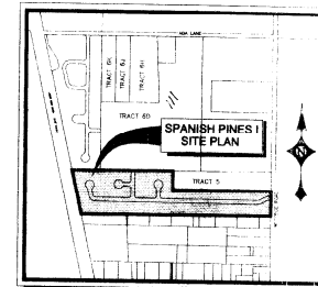
LOCATION MAP: 1" = 600'
